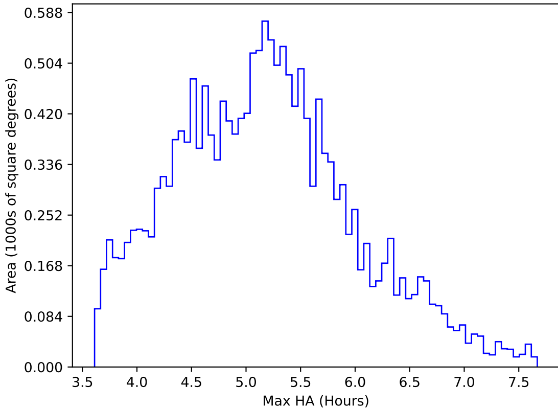
extra_ss_neo7_v3.4_10yrs WFD all bands: Max HA
