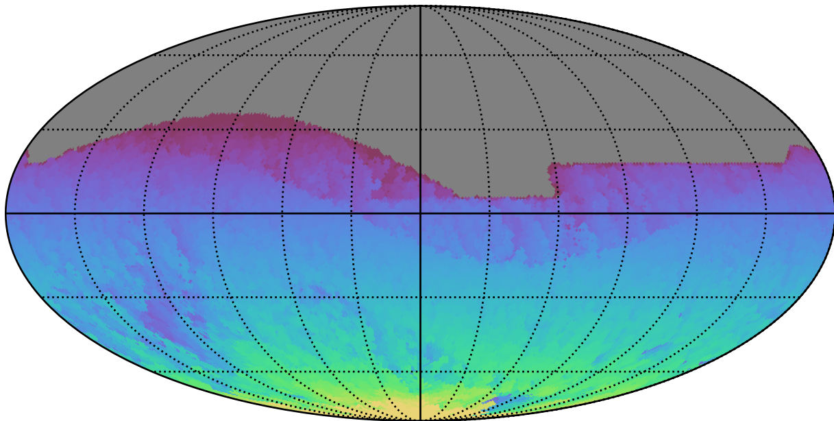
extra_ss_neo7_v3.4_10yrs All sky all bands: Max HA
