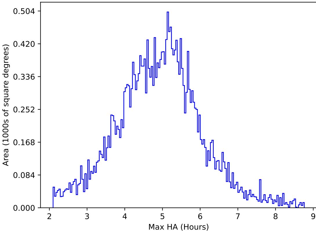
extra_ss_neo7_v3.4_10yrs All sky all bands: Max HA
