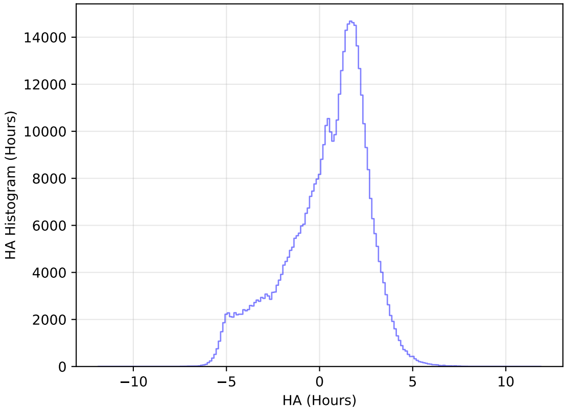
extra_ss_neo7_v3.4_10yrs WFD r band: HA Histogram
