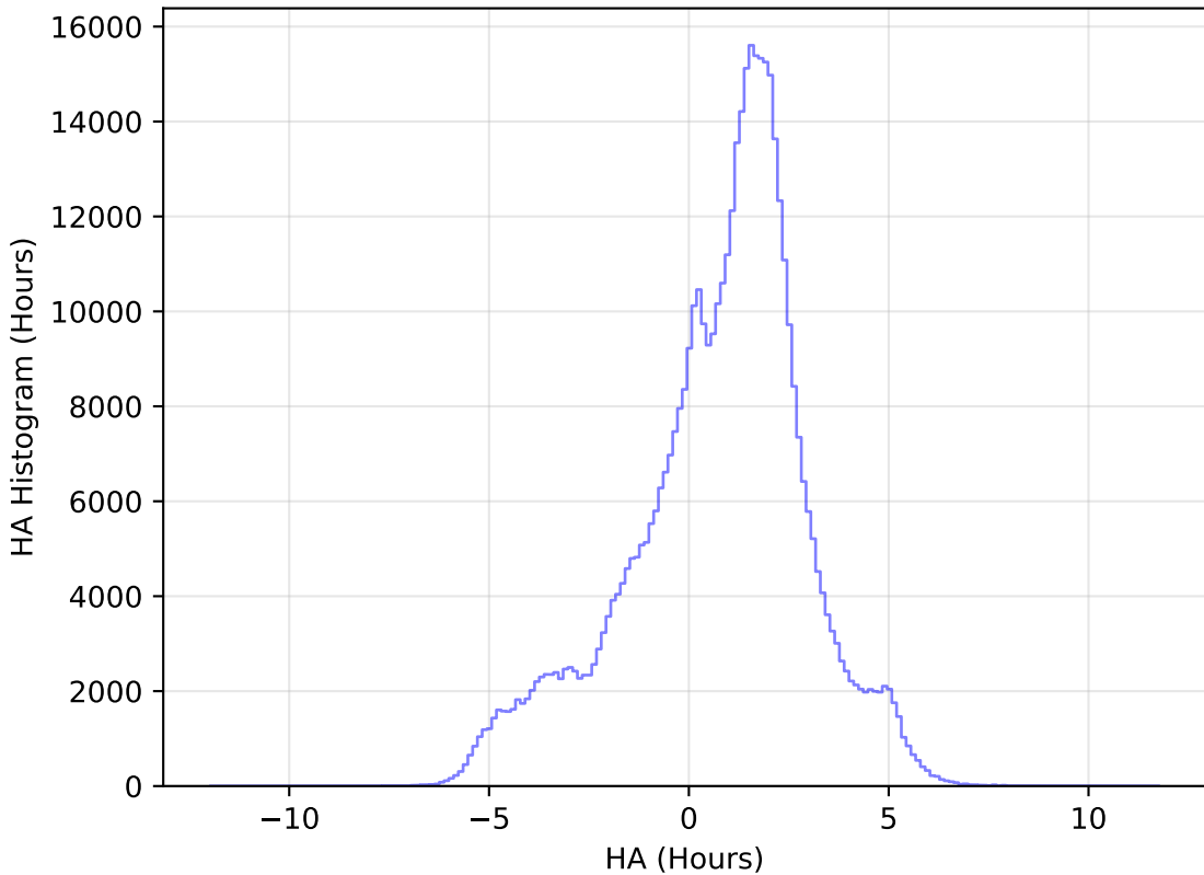
extra_ss_neo7_v3.4_10yrs WFD i band: HA Histogram
