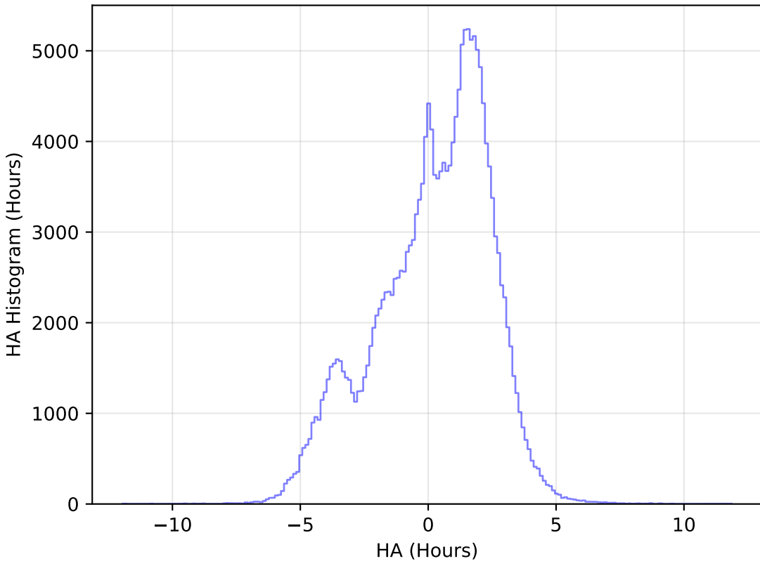
extra_ss_neo7_v3.4_10yrs WFD g band: HA Histogram
