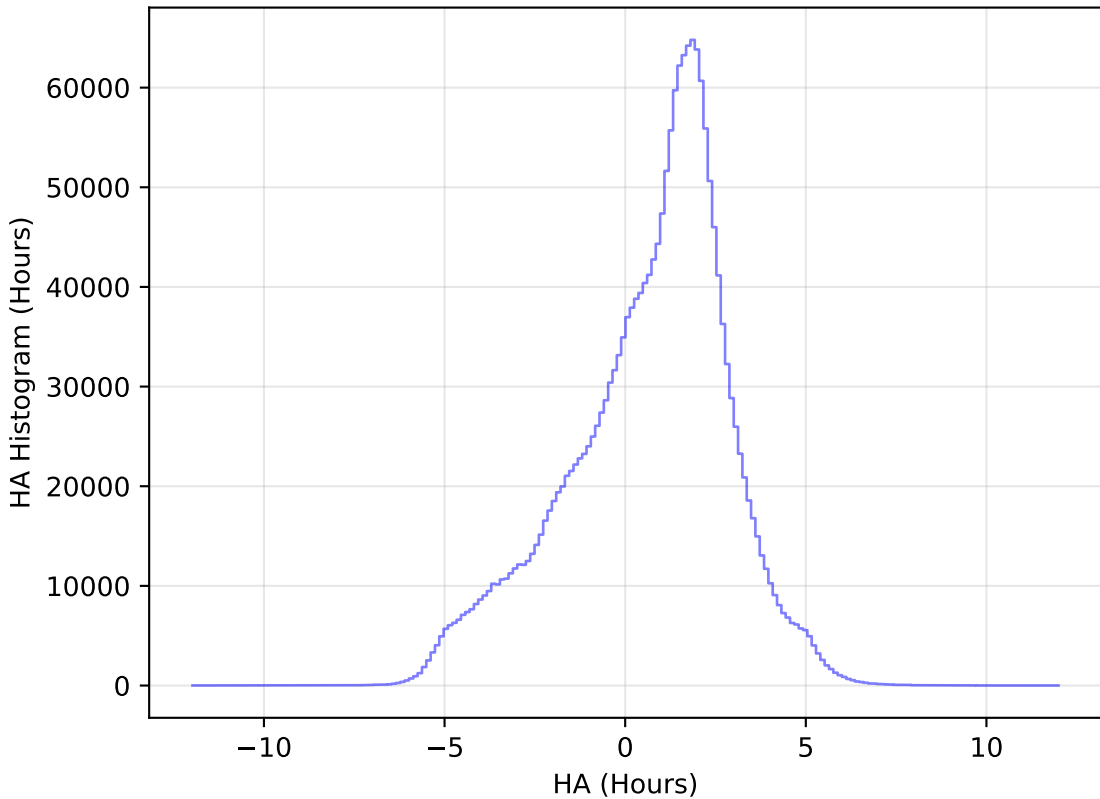
extra_ss_neo7_v3.4_10yrs WFD all bands: HA Histogram
