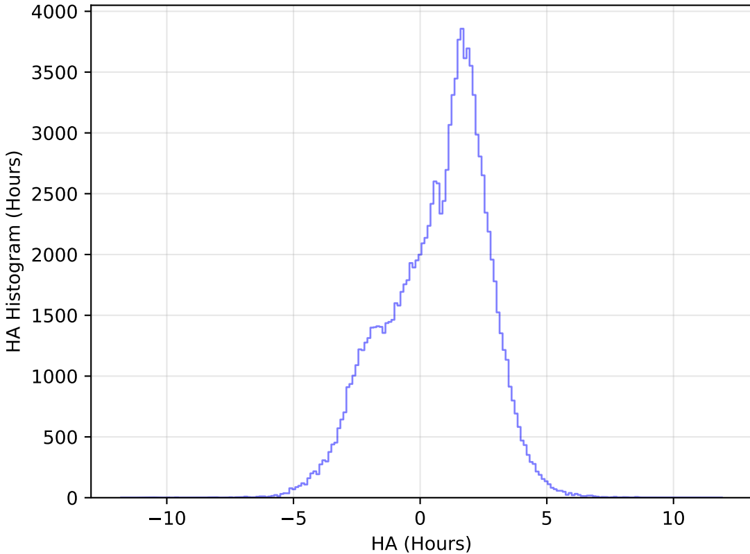
extra_ss_neo7_v3.4_10yrs All sky u band: HA Histogram
