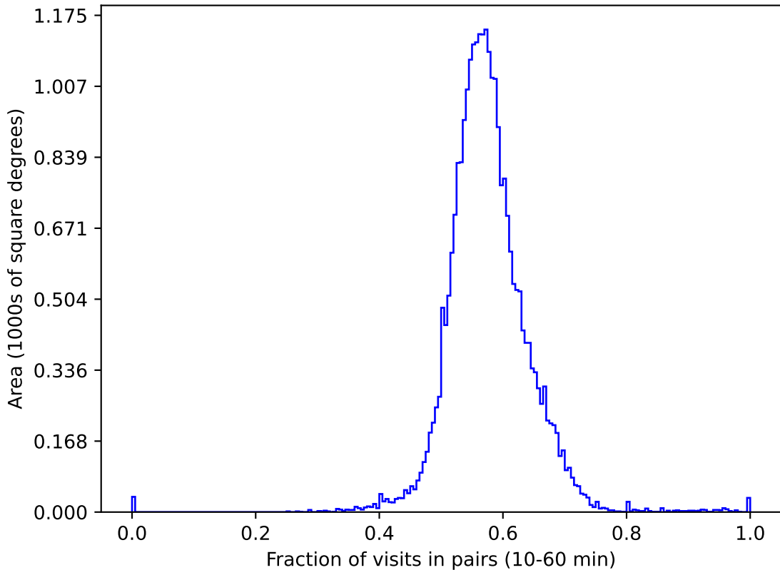
extra_ss_neo7_v3.4_10yrs gri All sky: Fraction of visits in pairs (10-60 min)
