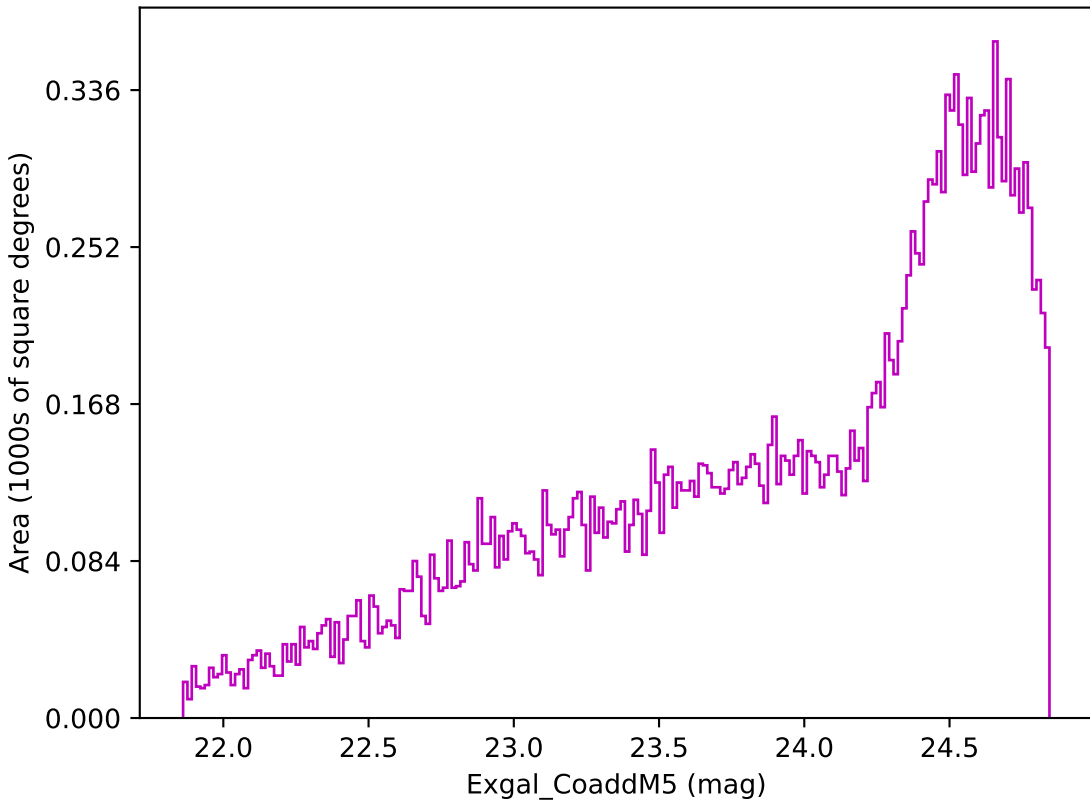
extra_ss_neo7_v3.4_10yrs Yr 3-4 z band: Exgal_CoaddM5
