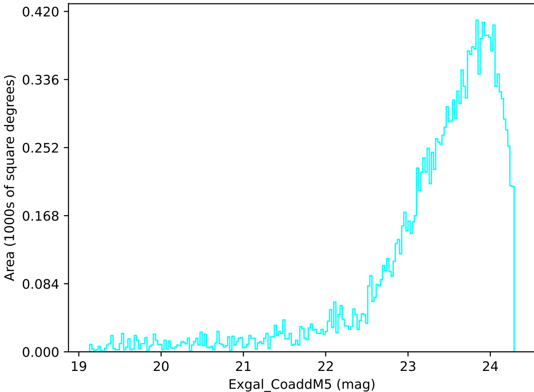
extra_ss_neo7_v3.4_10yrs Yr 3-4 u band: Exgal_CoaddM5
