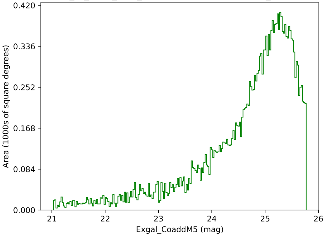
extra_ss_neo7_v3.4_10yrs Yr 3-4 g band: Exgal_CoaddM5
