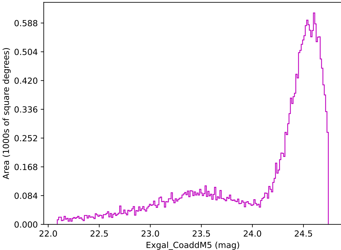
extra_ss_neo7_v3.4_10yrs Yr 1 z band: Exgal_CoaddM5
