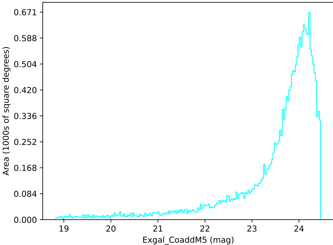
extra_ss_neo7_v3.4_10yrs Yr 1 u band: Exgal_CoaddM5
