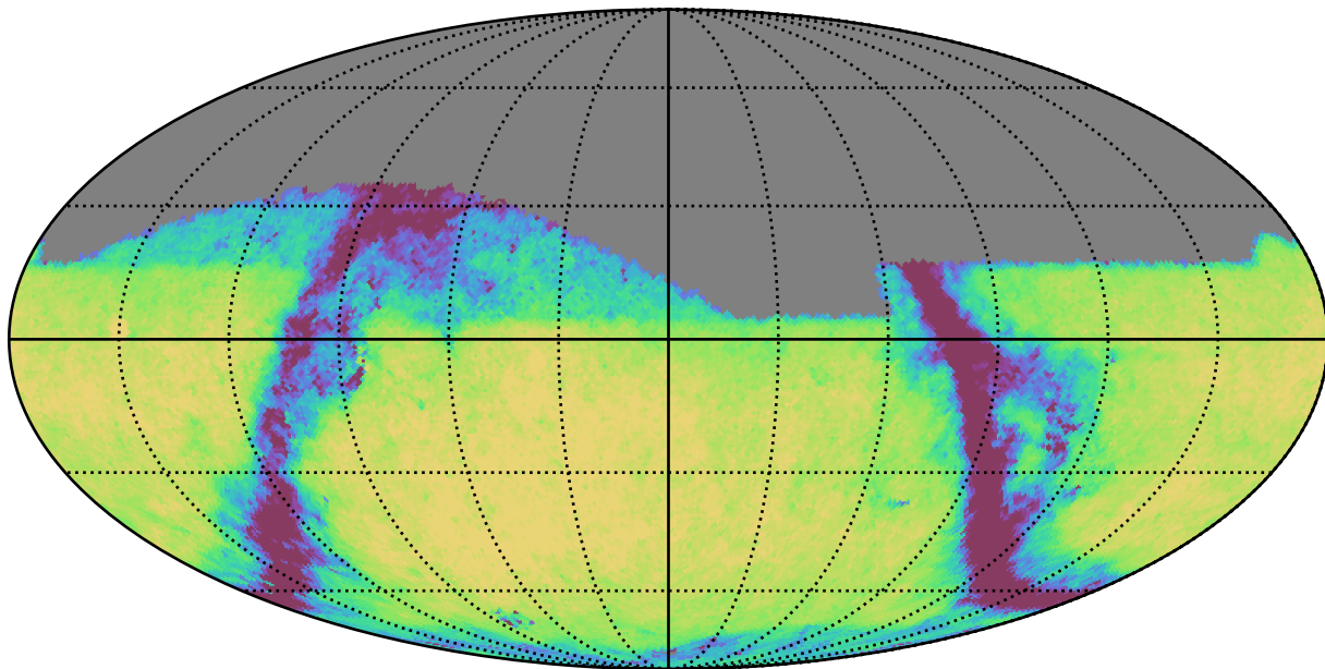
extra_ss_neo7_v3.4_10yrs Yr 1 r band: Exgal_CoaddM5
