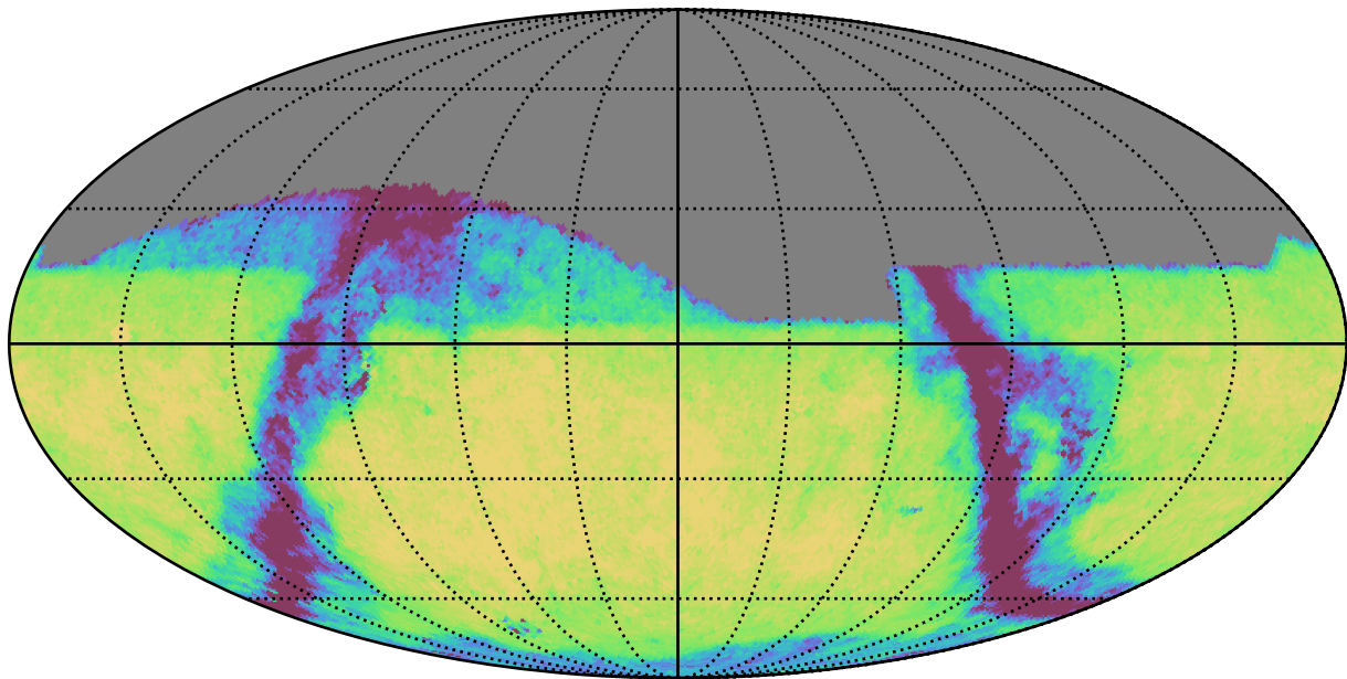
extra_ss_neo7_v3.4_10yrs Yr 1 i band: Exgal_CoaddM5
