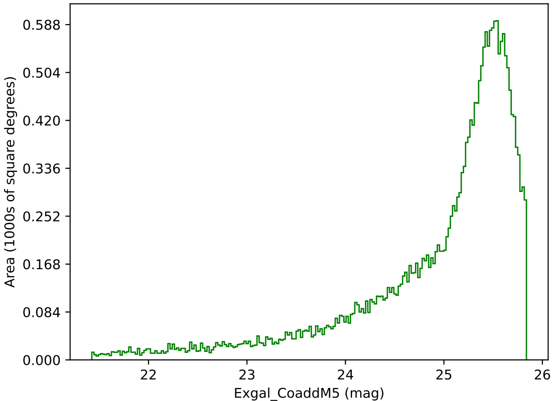
extra_ss_neo7_v3.4_10yrs Yr 1 g band: Exgal_CoaddM5
