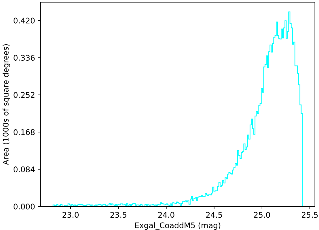
extra_ss_neo7_v3.4_10yrs WFD u band: Exgal_CoaddM5
