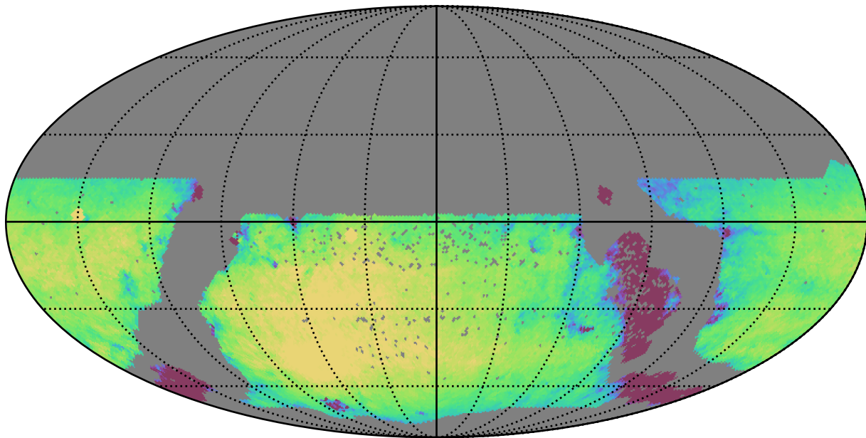
extra_ss_neo7_v3.4_10yrs WFD r band: Exgal_CoaddM5
