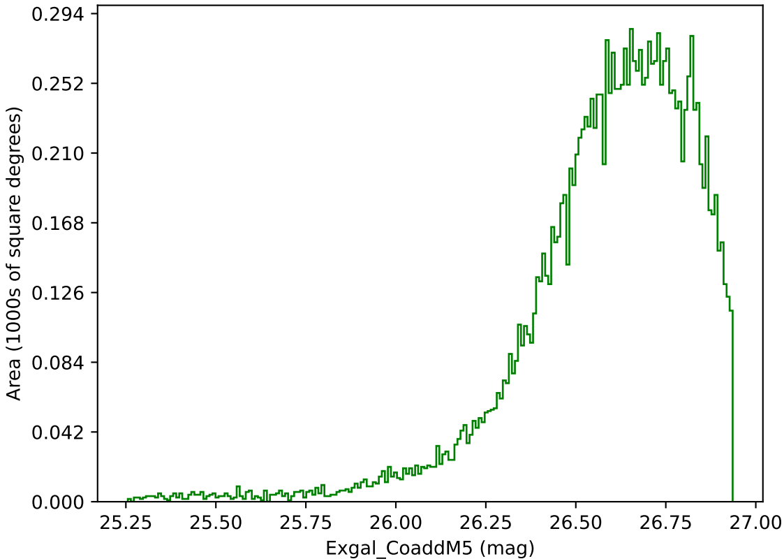
extra_ss_neo7_v3.4_10yrs WFD g band: Exgal_CoaddM5
