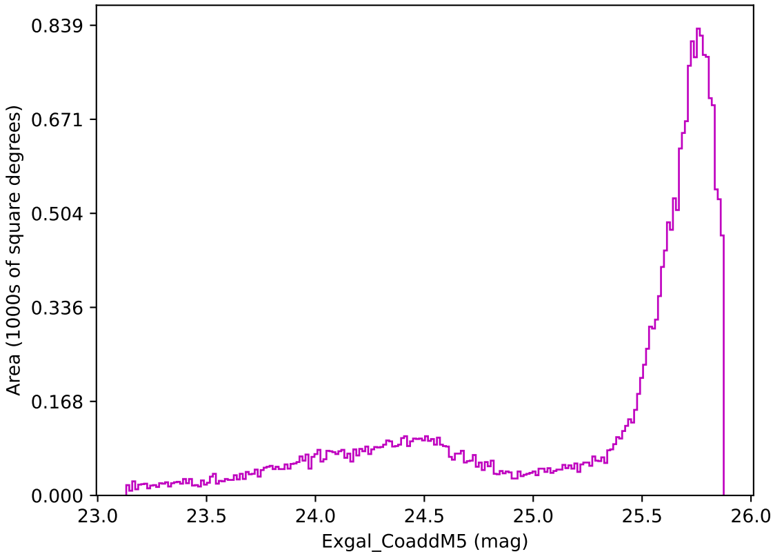
extra_ss_neo7_v3.4_10yrs All sky z band: Exgal_CoaddM5
