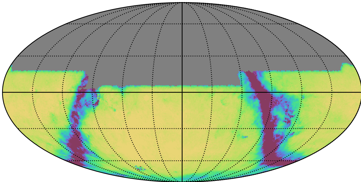
extra_ss_neo7_v3.4_10yrs All sky u band: Exgal_CoaddM5
