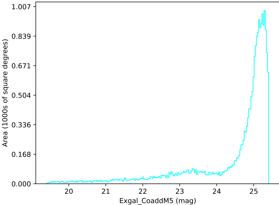
extra_ss_neo7_v3.4_10yrs All sky u band: Exgal_CoaddM5
