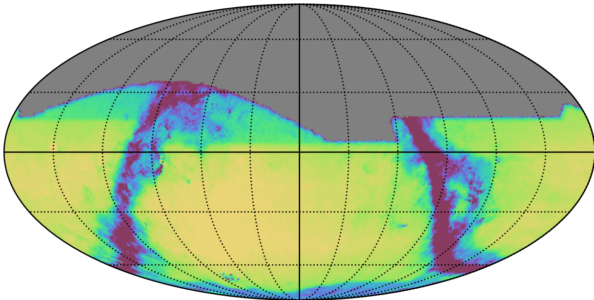
extra_ss_neo7_v3.4_10yrs All sky r band: Exgal_CoaddM5
