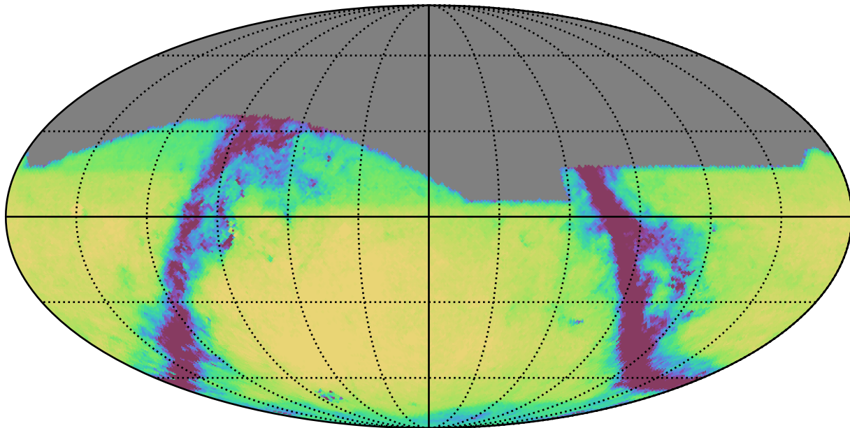
extra_ss_neo7_v3.4_10yrs All sky g band: Exgal_CoaddM5
