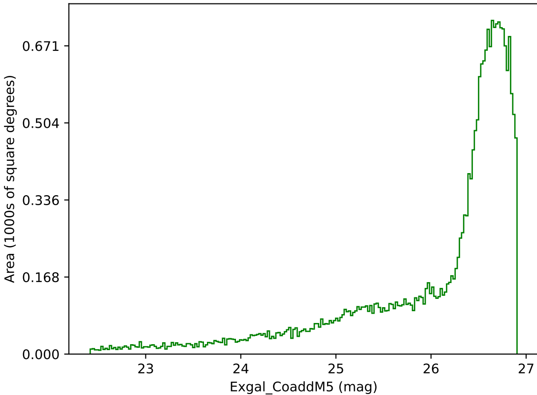
extra_ss_neo7_v3.4_10yrs All sky g band: Exgal_CoaddM5
