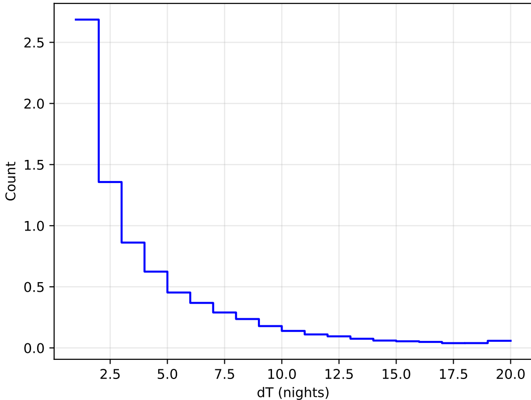
extra_ss_neo7_v3.4_10yrs WFD all bands: DeltaNight Histogram 1e6
