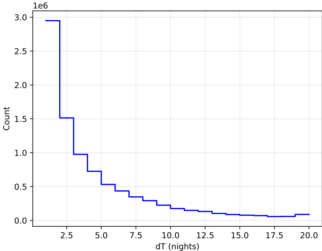
extra_ss_neo7_v3.4_10yrs All sky all bands: DeltaNight Histogram
