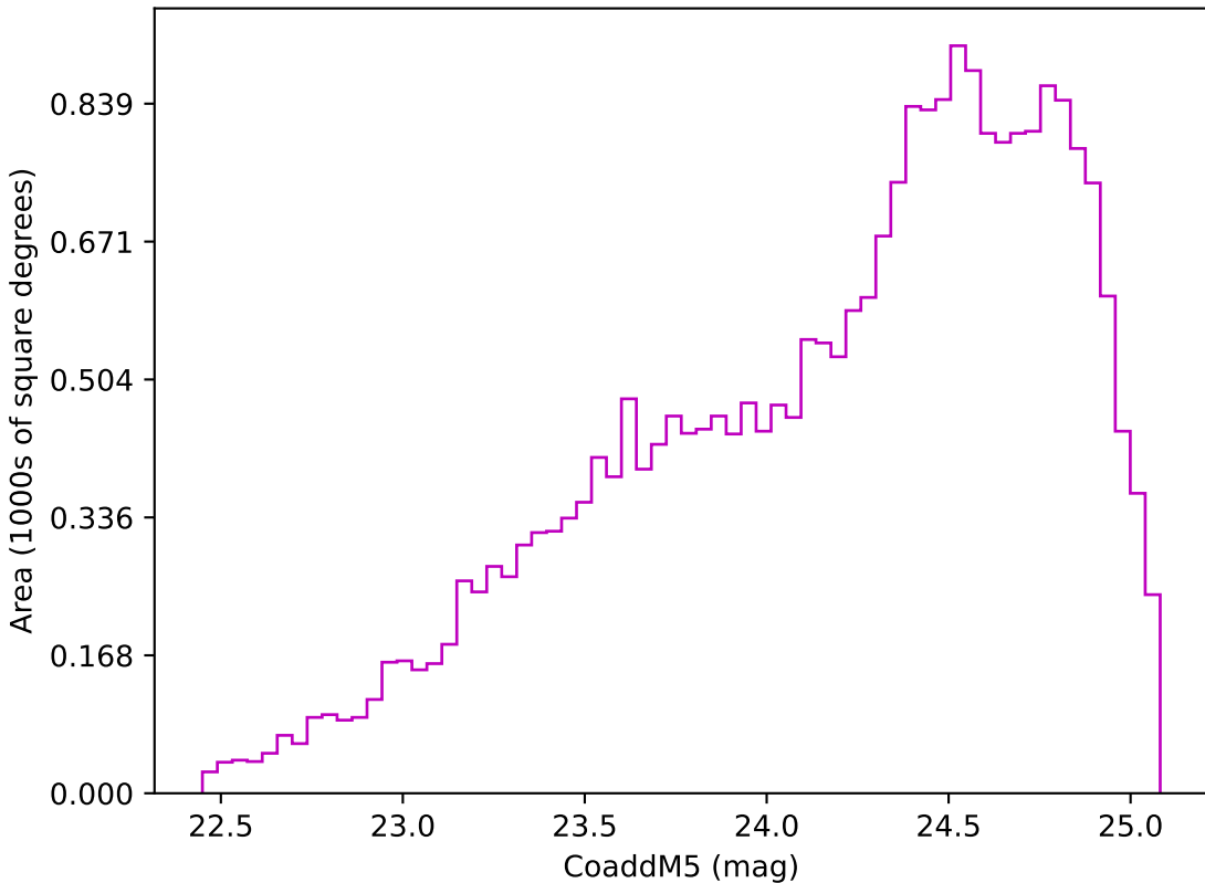
extra_ss_neo7_v3.4_10yrs Yr 3-4 z band: CoaddM5
