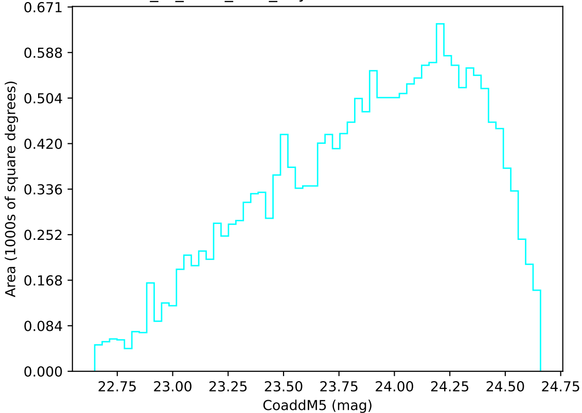
extra_ss_neo7_v3.4_10yrs Yr 3-4 u band: CoaddM5
