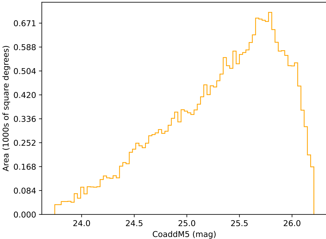
extra_ss_neo7_v3.4_10yrs Yr 3-4 r band: CoaddM5
