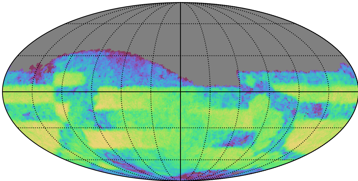
extra_ss_neo7_v3.4_10yrs Yr 3-4 i band: CoaddM5
