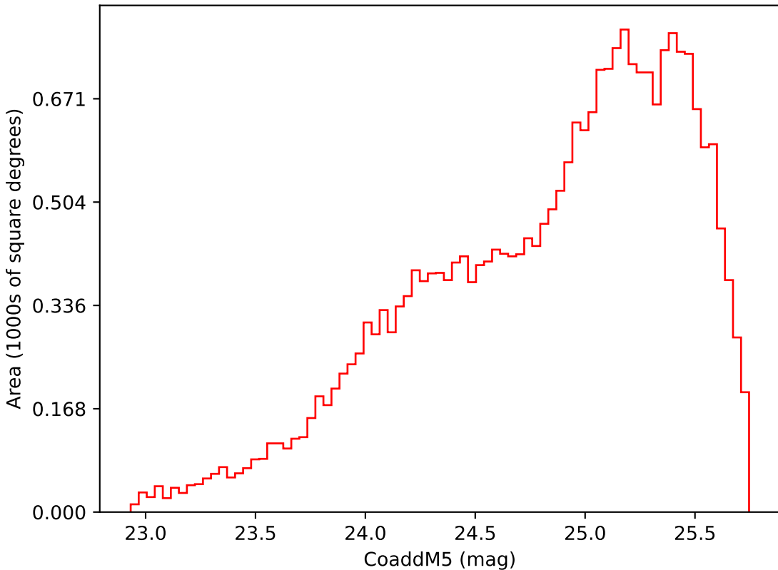
extra_ss_neo7_v3.4_10yrs Yr 3-4 i band: CoaddM5
