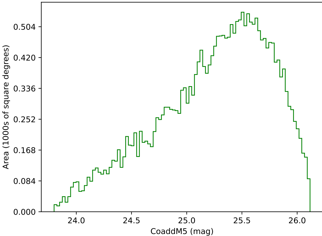
extra_ss_neo7_v3.4_10yrs Yr 3-4 g band: CoaddM5
