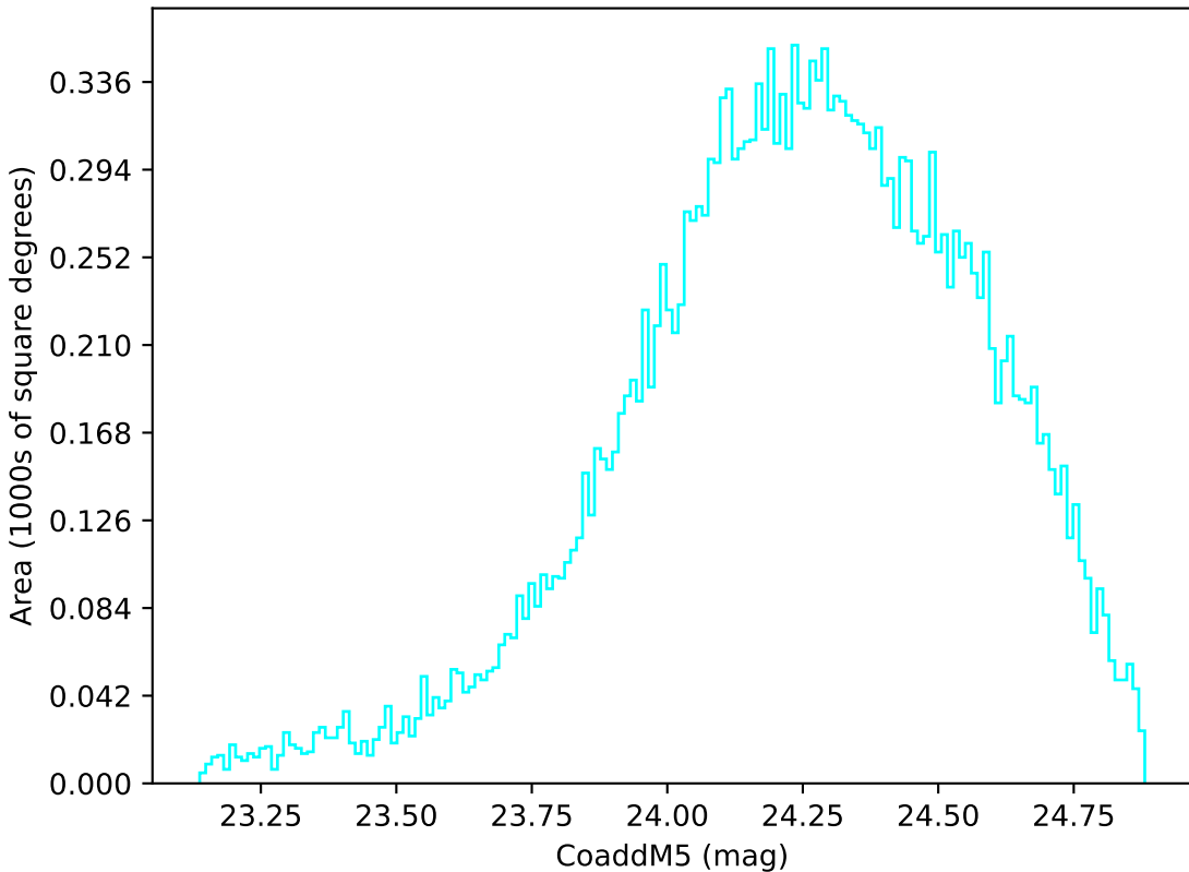
extra_ss_neo7_v3.4_10yrs Yr 1 u band: CoaddM5
