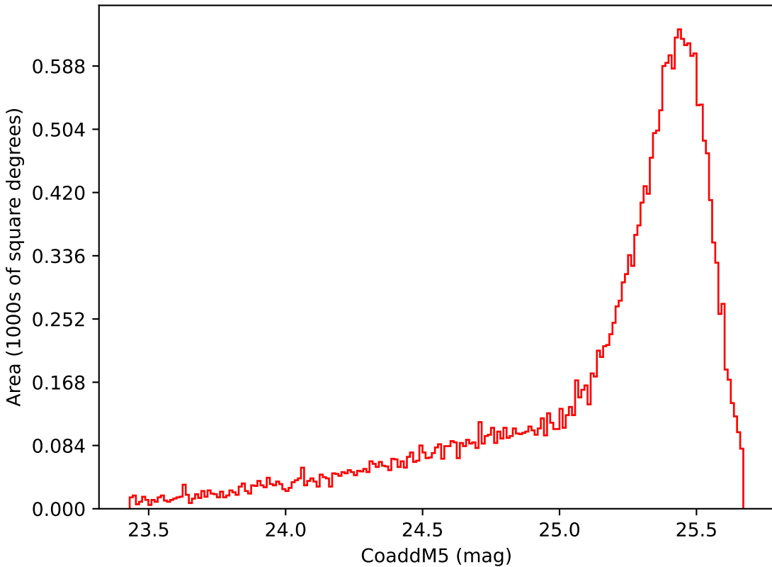
extra_ss_neo7_v3.4_10yrs Yr 1 i band: CoaddM5
