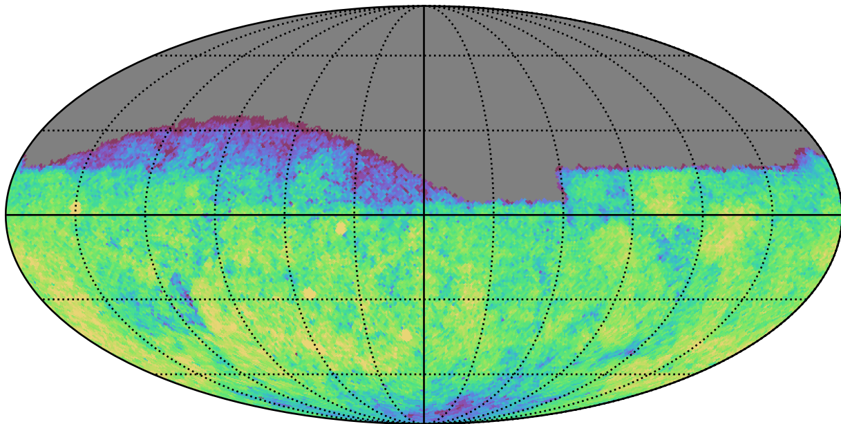
extra_ss_neo7_v3.4_10yrs Yr 1 g band: CoaddM5
