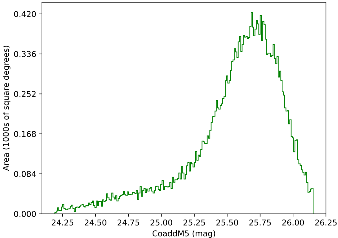
extra_ss_neo7_v3.4_10yrs Yr 1 g band: CoaddM5
