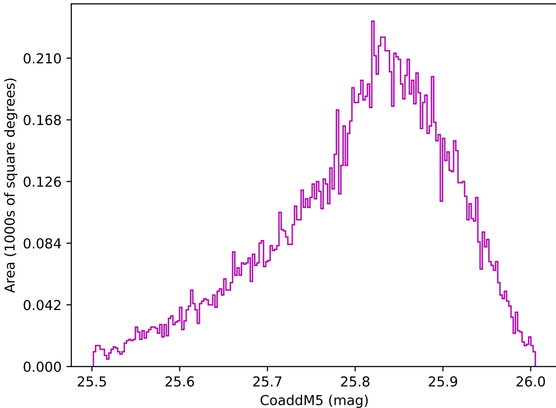
extra_ss_neo7_v3.4_10yrs WFD z band: CoaddM5
