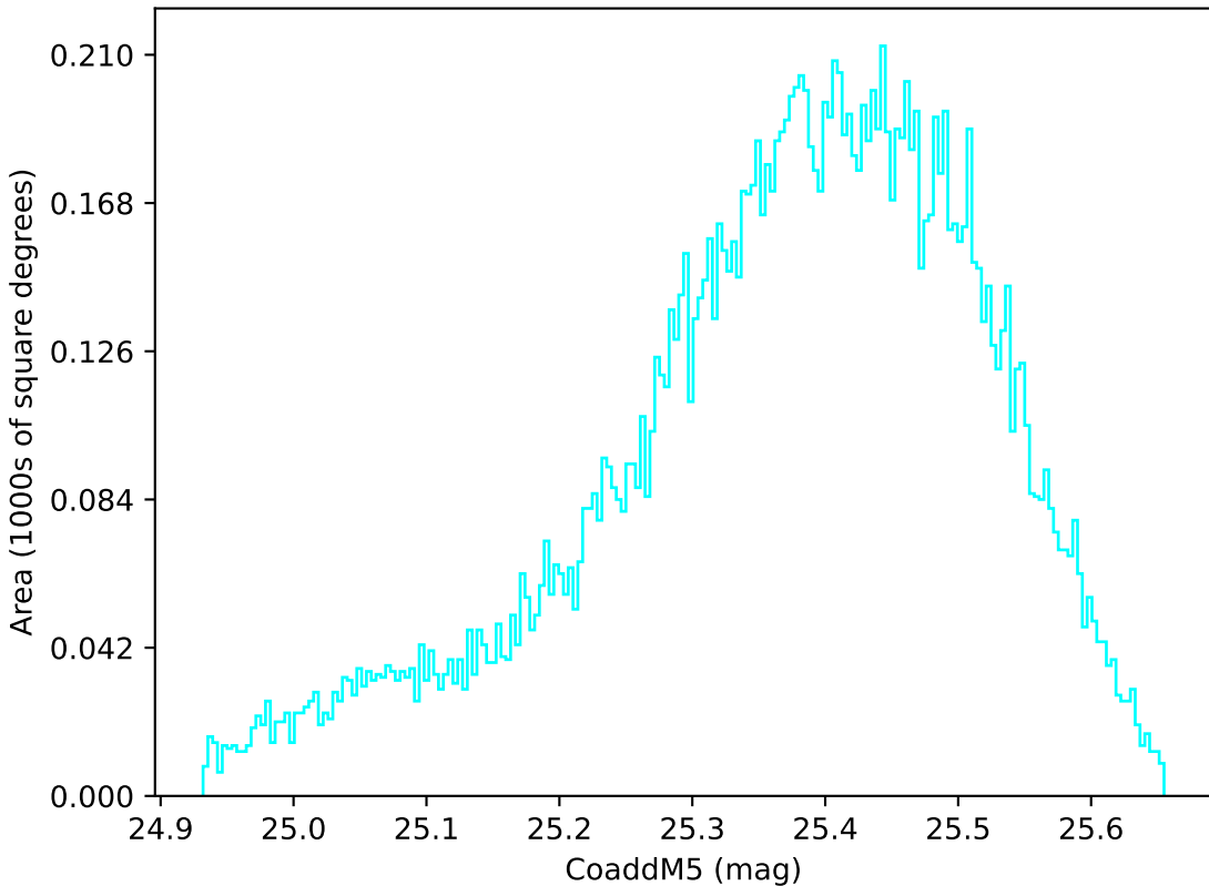
extra_ss_neo7_v3.4_10yrs WFD u band: CoaddM5
