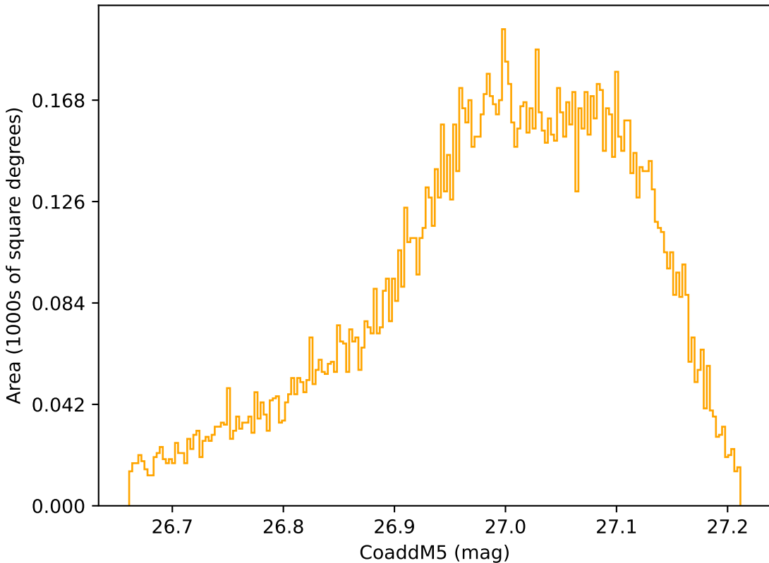
extra_ss_neo7_v3.4_10yrs WFD r band: CoaddM5
