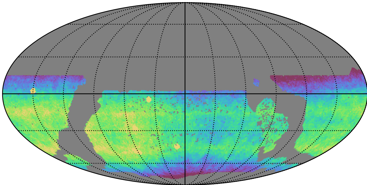
extra_ss_neo7_v3.4_10yrs WFD i band: CoaddM5
