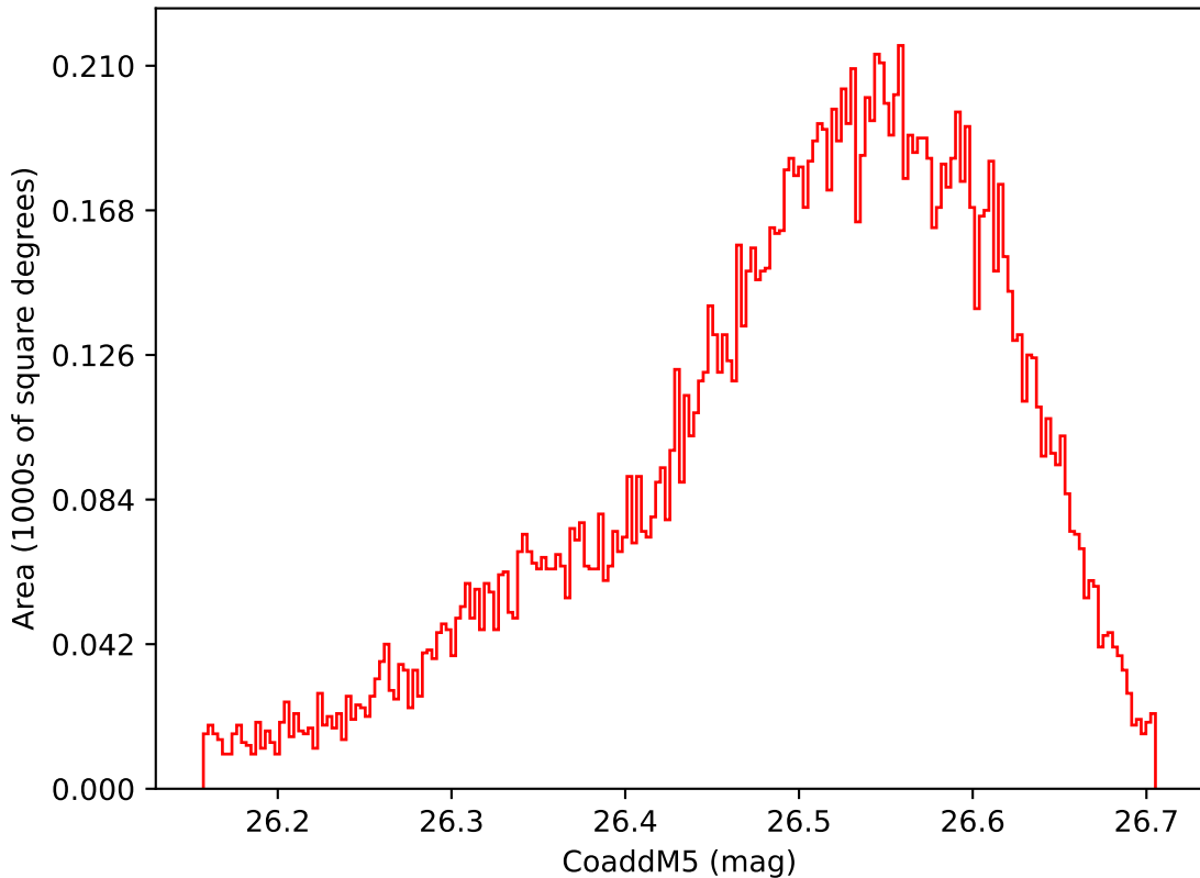
extra_ss_neo7_v3.4_10yrs WFD i band: CoaddM5
