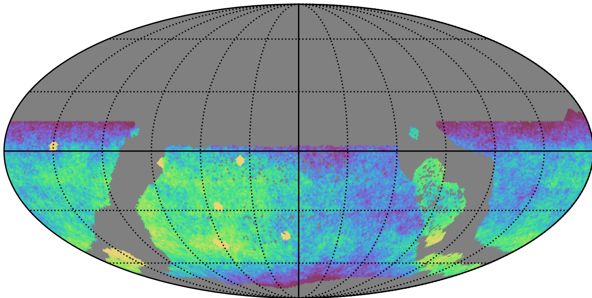
extra_ss_neo7_v3.4_10yrs WFD g band: CoaddM5
