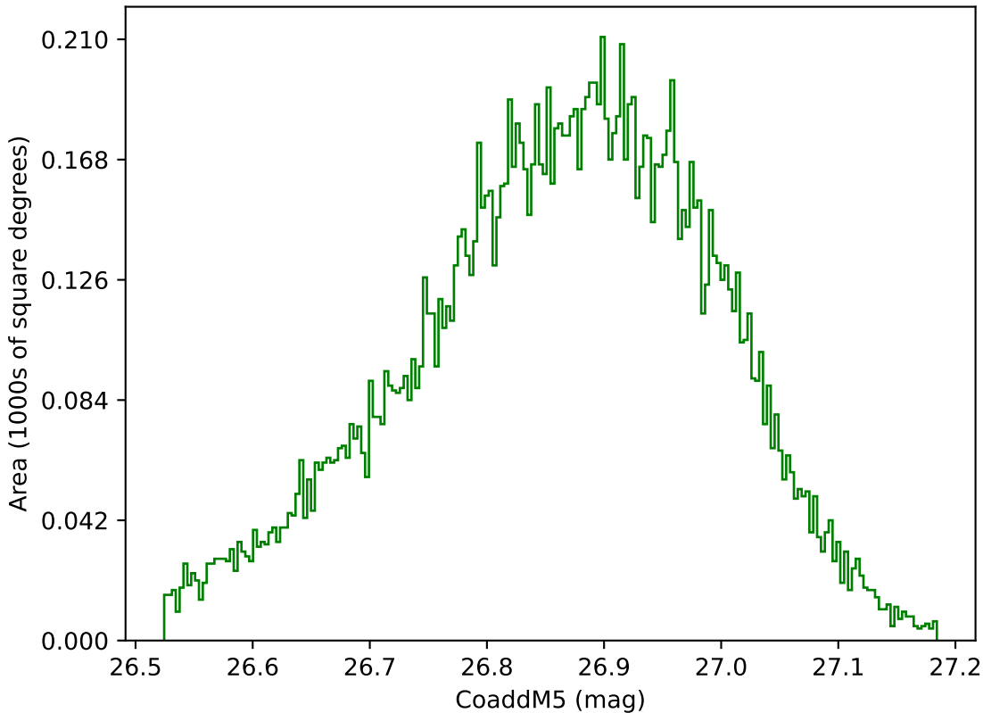
extra_ss_neo7_v3.4_10yrs WFD g band: CoaddM5
