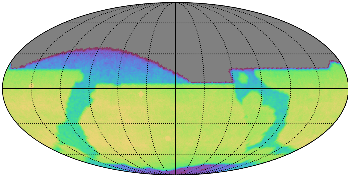
extra_ss_neo7_v3.4_10yrs All sky z band: CoaddM5
