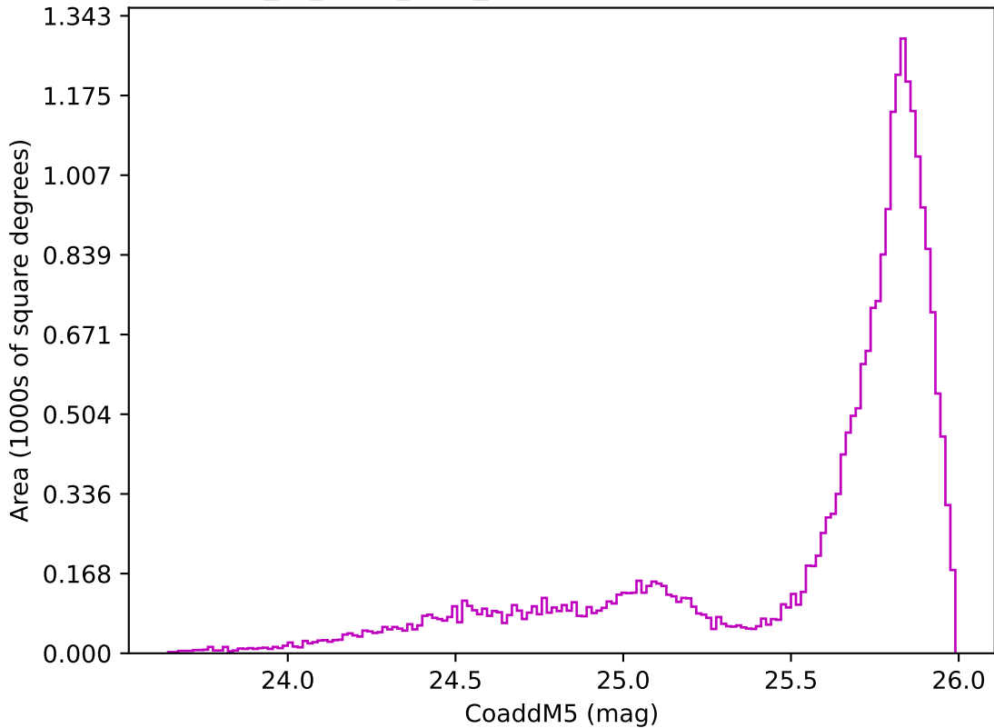
extra_ss_neo7_v3.4_10yrs All sky z band: CoaddM5
