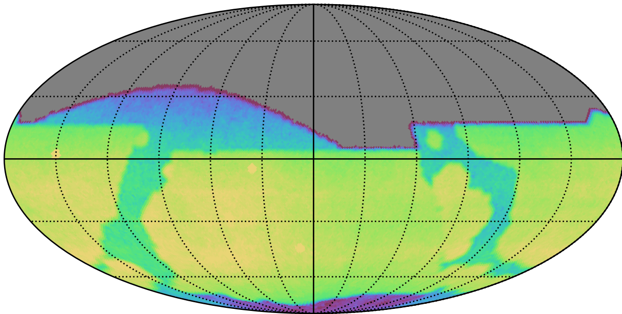
extra_ss_neo7_v3.4_10yrs All sky r band: CoaddM5
