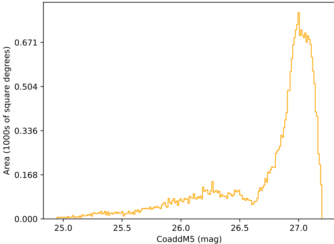
extra_ss_neo7_v3.4_10yrs All sky r band: CoaddM5
