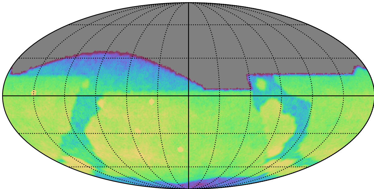
extra_ss_neo7_v3.4_10yrs All sky g band: CoaddM5
